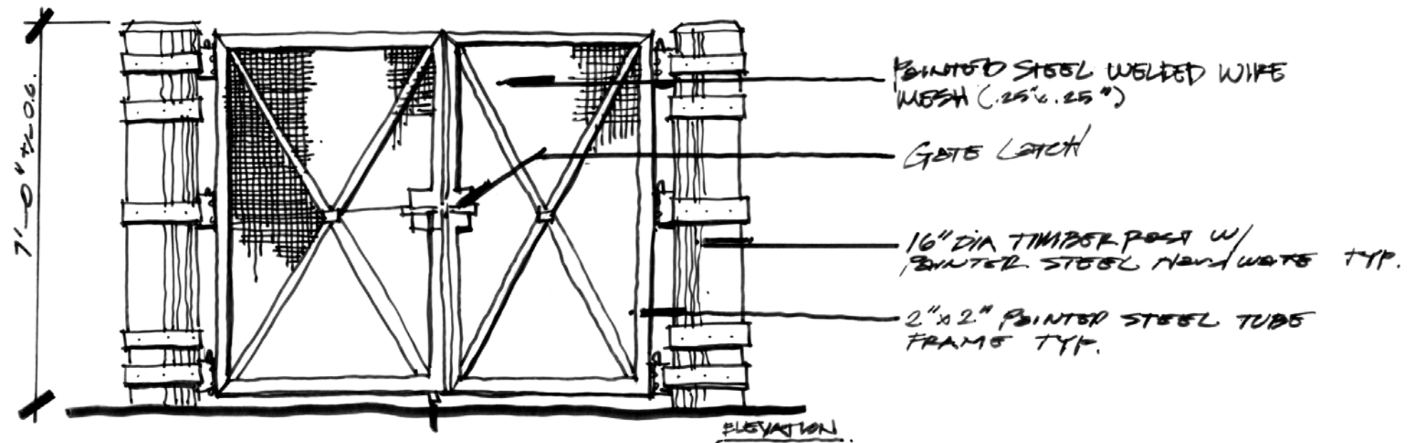
TRASH ENCLOSURE DETAIL NTS
